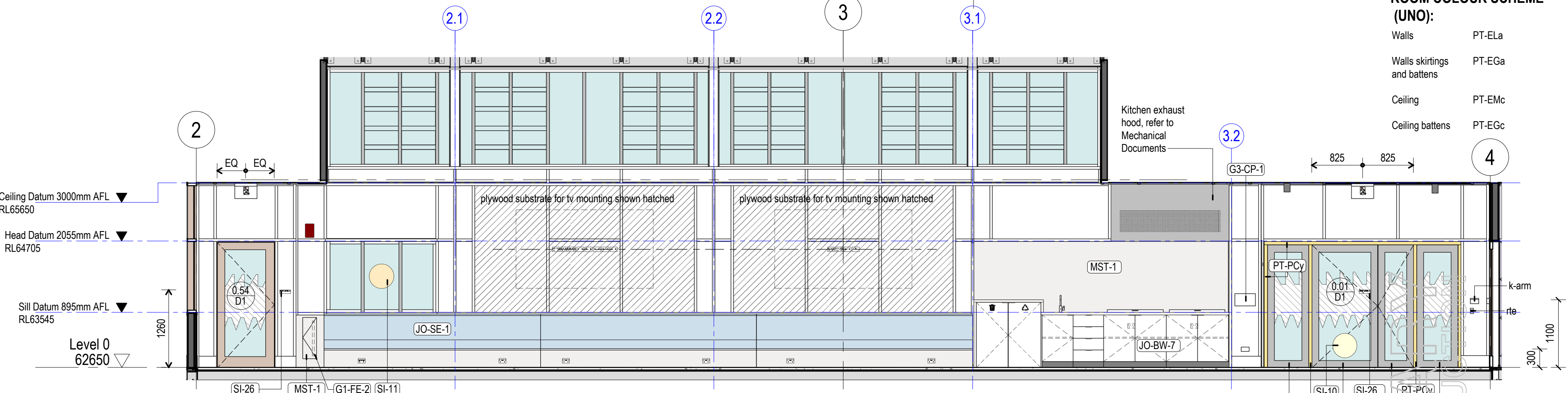
4 0.02 - Covered Outdoor - East Elevation 1 : 50
