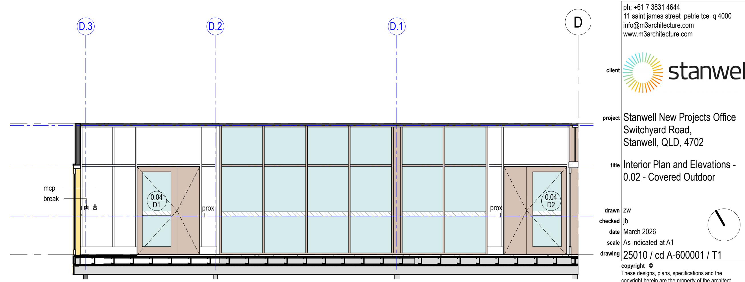
7 0.02 - Covered Outdoor - South Elevation 1 1 : 50
