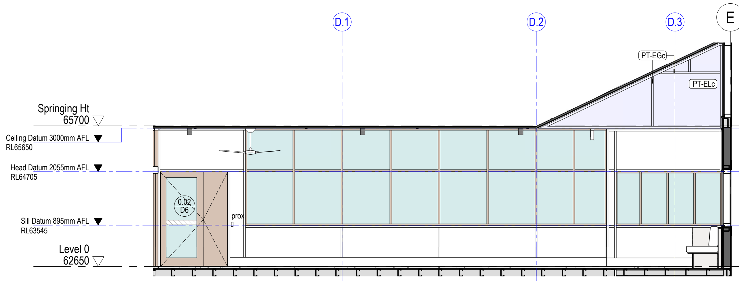
2 0.02 - Covered Outdoor - North Elevation 1 1 : 50
