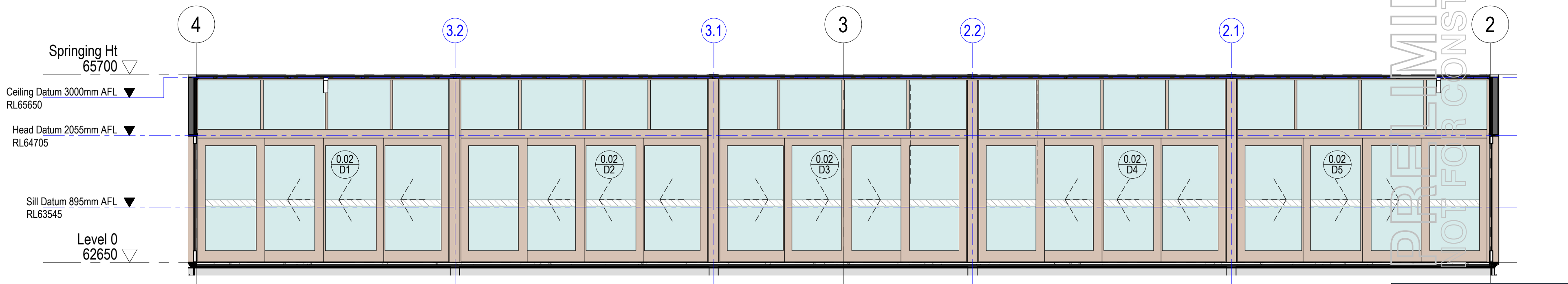
5 0.02 - Covered Outdoor - West Elevation 1 : 50
