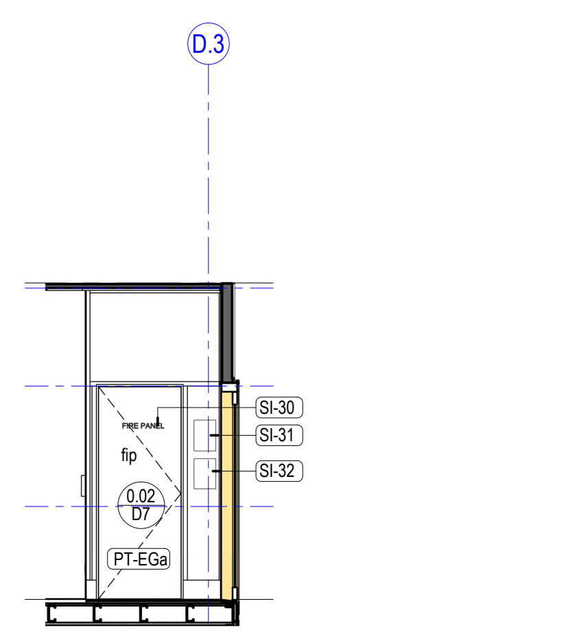
3 0.02 - Covered Outdoor - North Elevation 2 1 : 50
